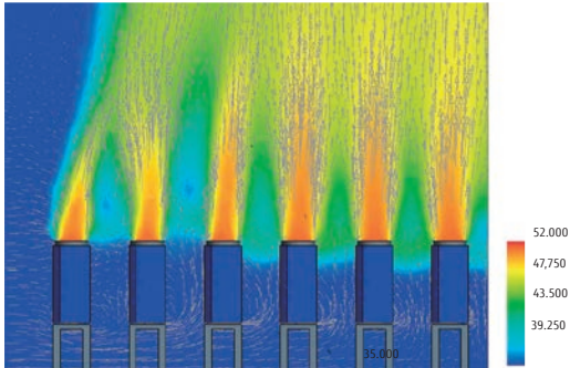
CFD Simulation
