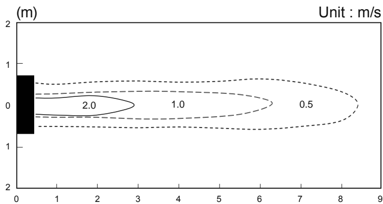
TOP VIEW Vertical airflow direction louver: Up Horizontal airflow direction louver: Center
