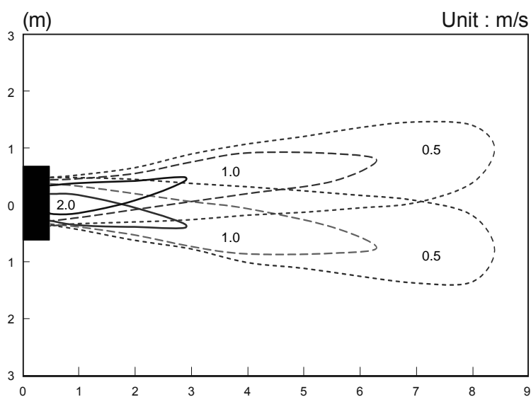
TOP VIEW Vertical airflow direction louver: Up Horizontal airflow direction louver: Right & Left
